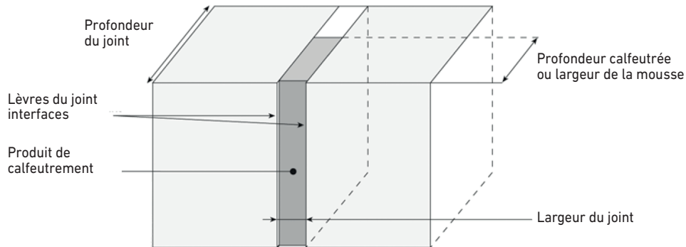
Figure 1 : Terminologie relative aux joints
